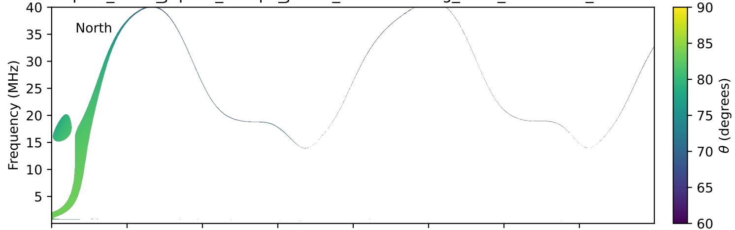
expres_earth_jupiter_europa_jrm33_lossc-wid1deg_3kev_20221019_v11.cdf
