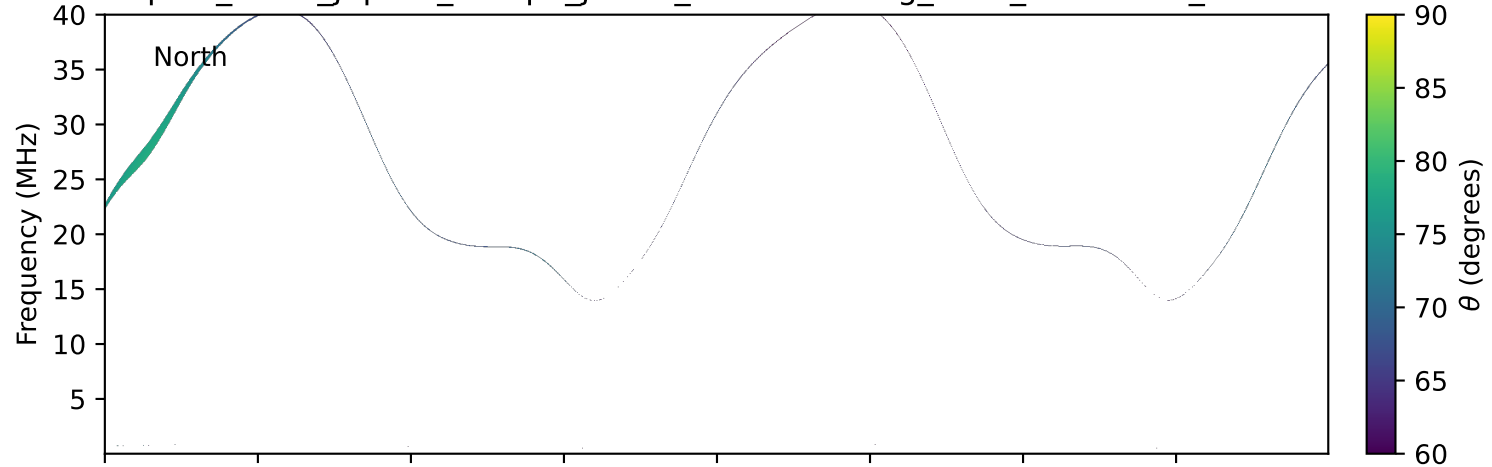
expres_earth_jupiter_europa_jrm33_lossc-wid1deg_3kev_20221012_v11.cdf
