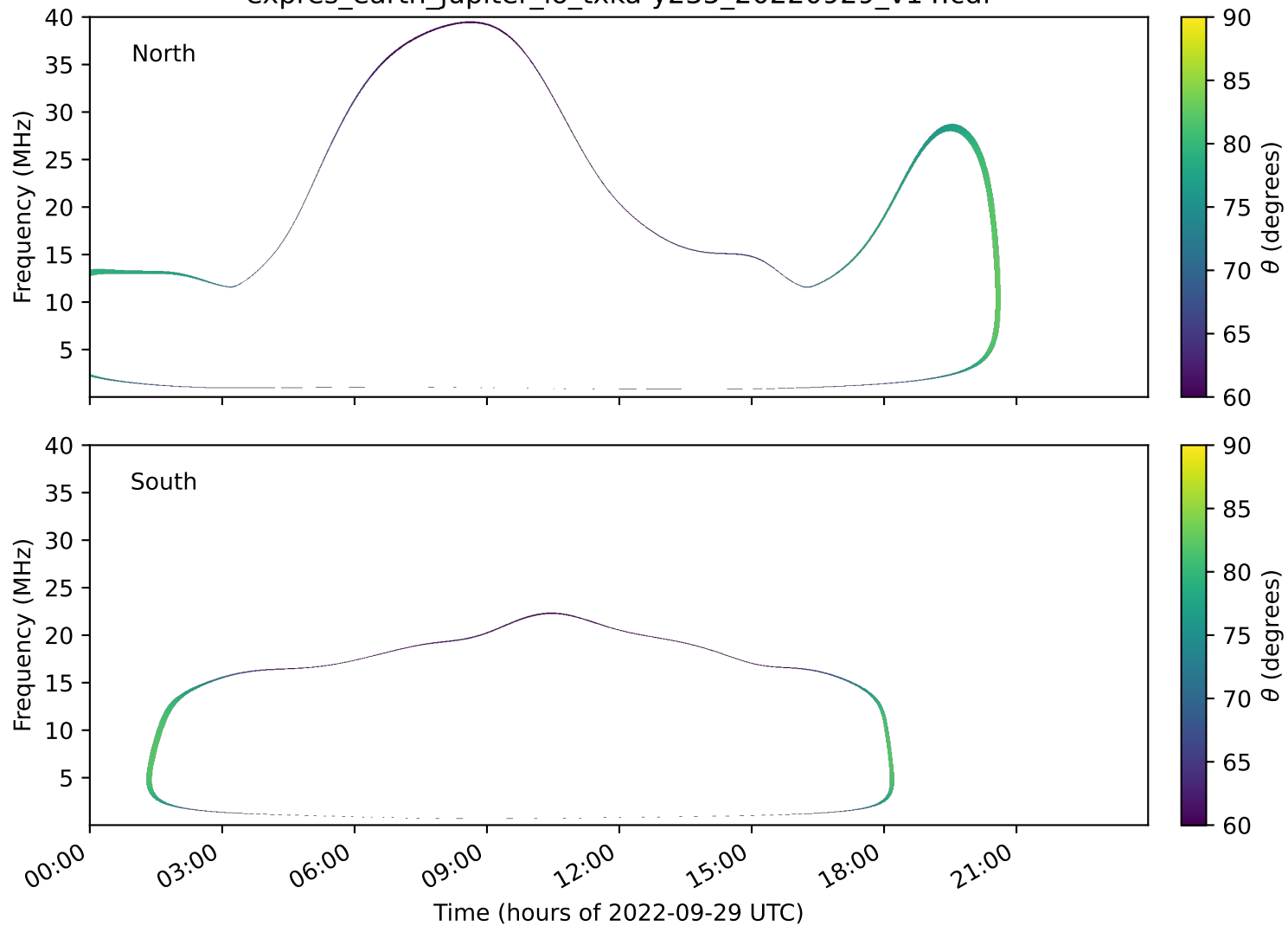
expres_earth_jupiter_io_txka-y235_20220929_v14.cdf
