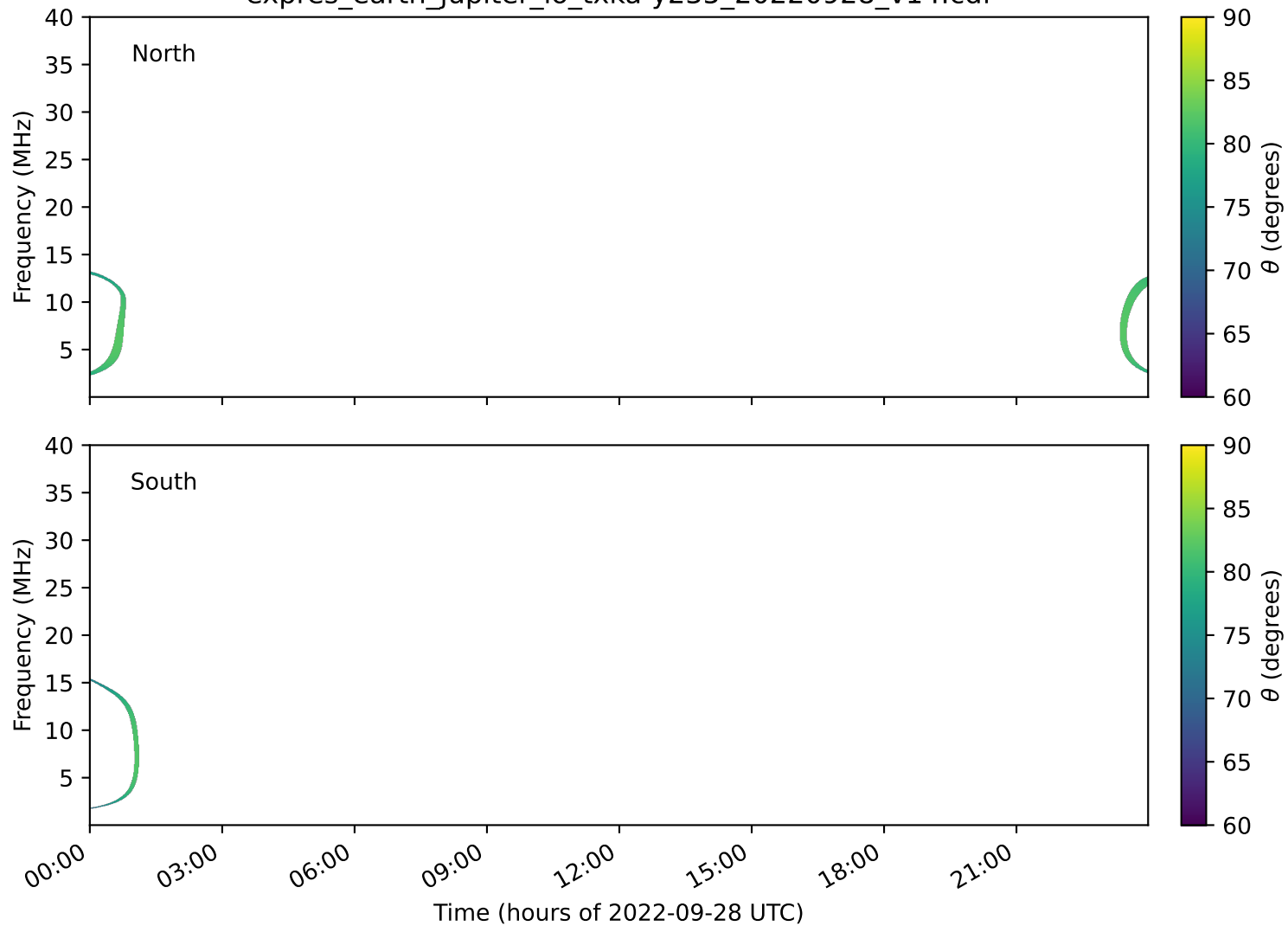
expres_earth_jupiter_io_txka-y235_20220928_v14.cdf
