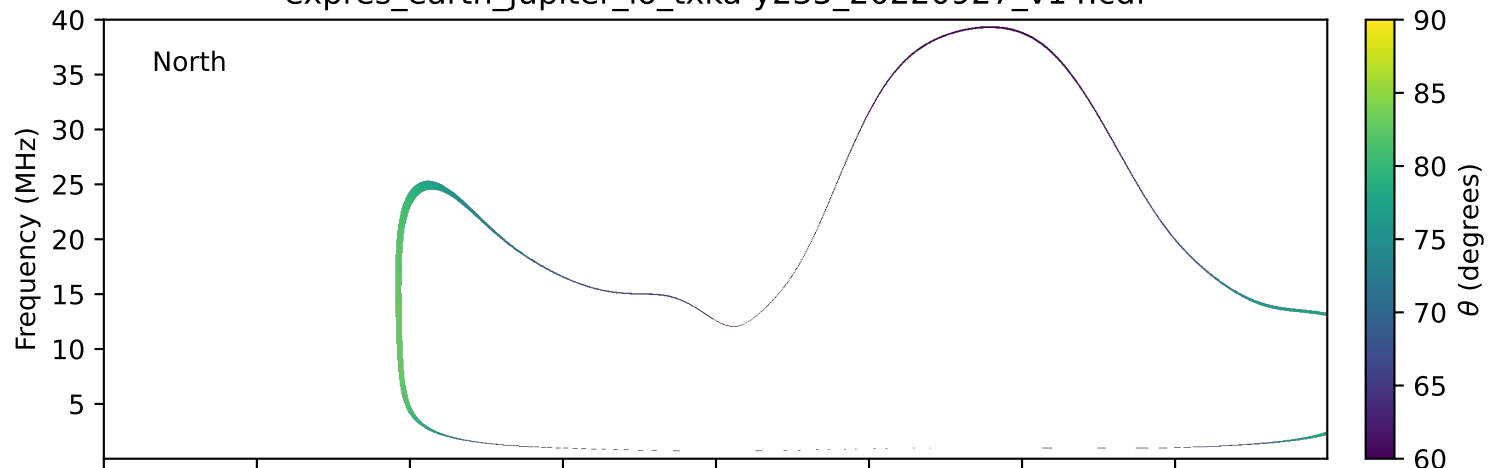
expres_earth_jupiter_io_txka-y235_20220927_v14.cdf
