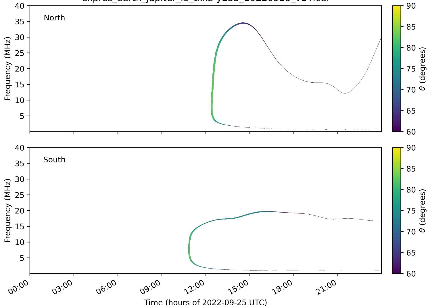
expres_earth_jupiter_io_txka-y235_20220925_v14.cdf
