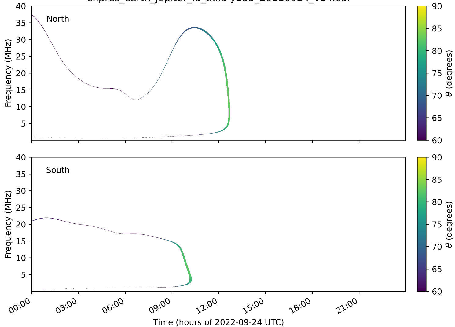
expres_earth_jupiter_io_txka-y235_20220924_v14.cdf
