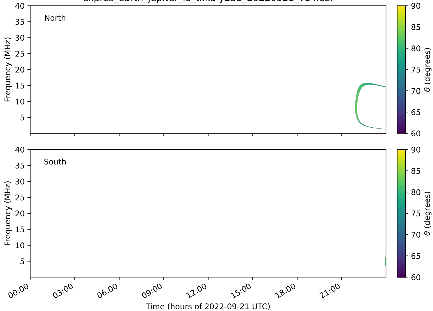
expres_earth_jupiter_io_txka-y235_20220921_v14.cdf
