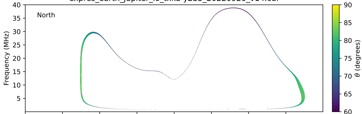
expres_earth_jupiter_io_txka-y235_20220920_v14.cdf
