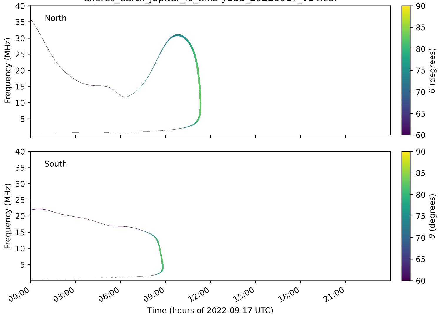
expres_earth_jupiter_io_txka-y235_20220917_v14.cdf
