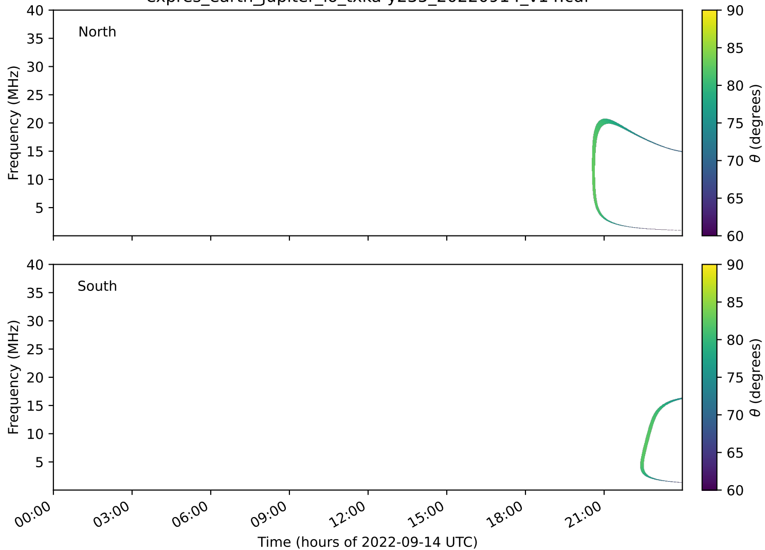
expres_earth_jupiter_io_txka-y235_20220914_v14.cdf
