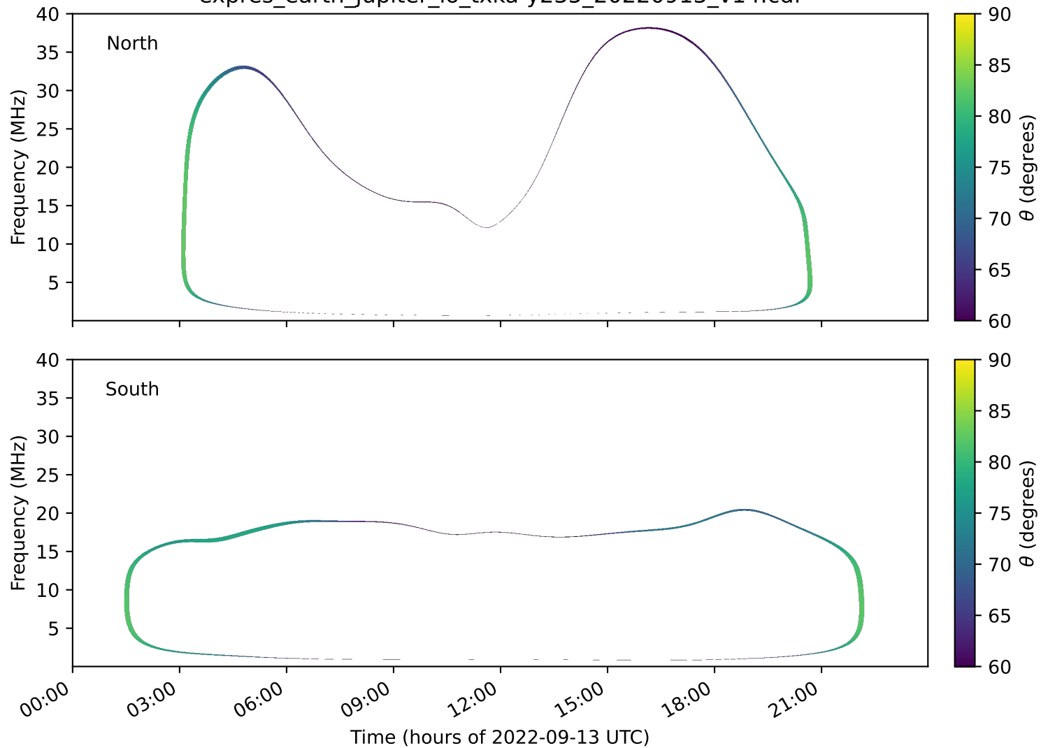
expres_earth_jupiter_io_txka-y235_20220913_v14.cdf
