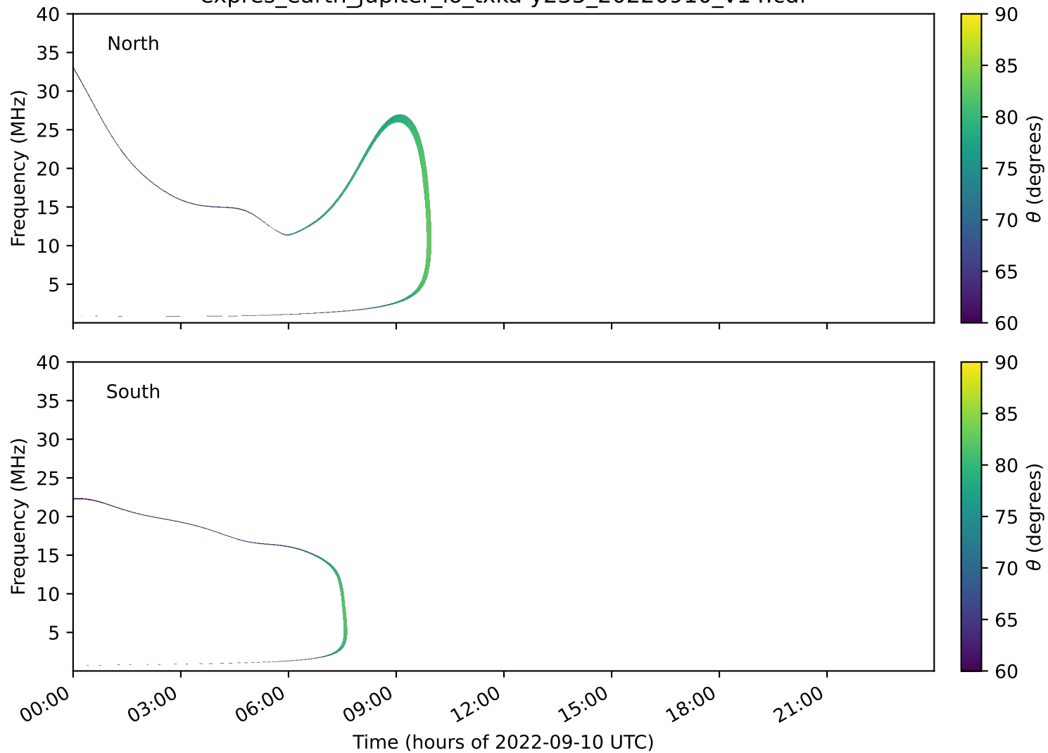
expres_earth_jupiter_io_txka-y235_20220910_v14.cdf
