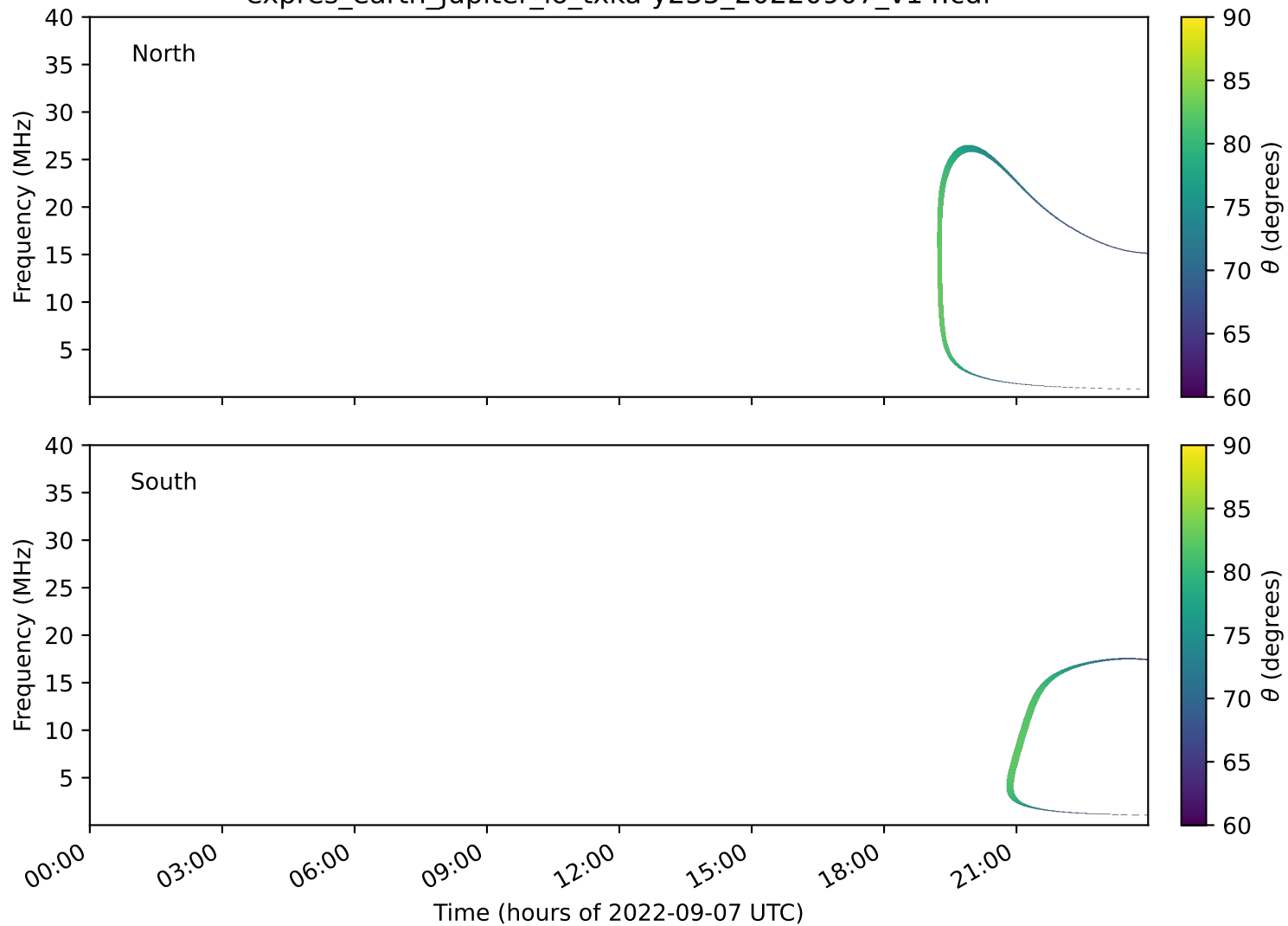
expres_earth_jupiter_io_txka-y235_20220907_v14.cdf
