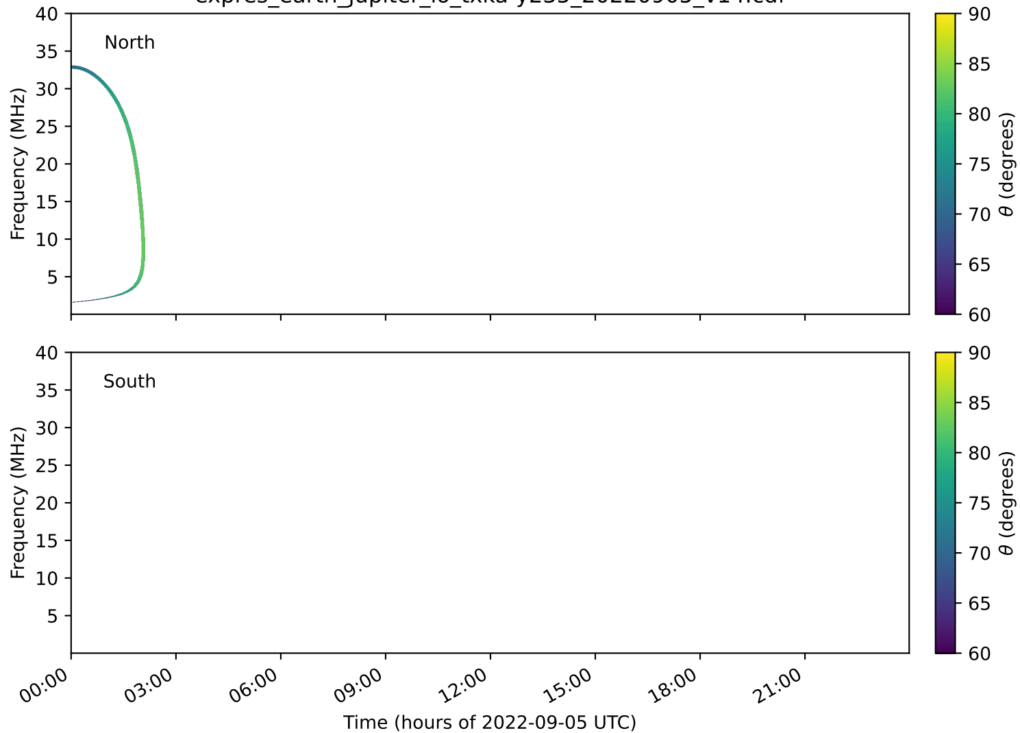
expres_earth_jupiter_io_txka-y235_20220905_v14.cdf
