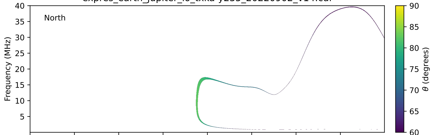
expres_earth_jupiter_io_txka-y235_20220902_v14.cdf
