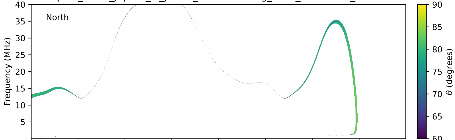
expres_earth_jupiter_io_jrm33_lossc-wid1deg_3kev_20220929_v11.cdf
