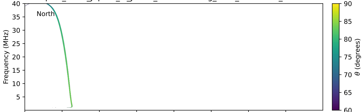
expres_earth_jupiter_io_jrm33_lossc-wid1deg_3kev_20220912_v11.cdf
