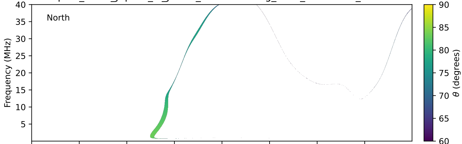
expres_earth_jupiter_io_jrm33_lossc-wid1deg_3kev_20220911_v11.cdf
