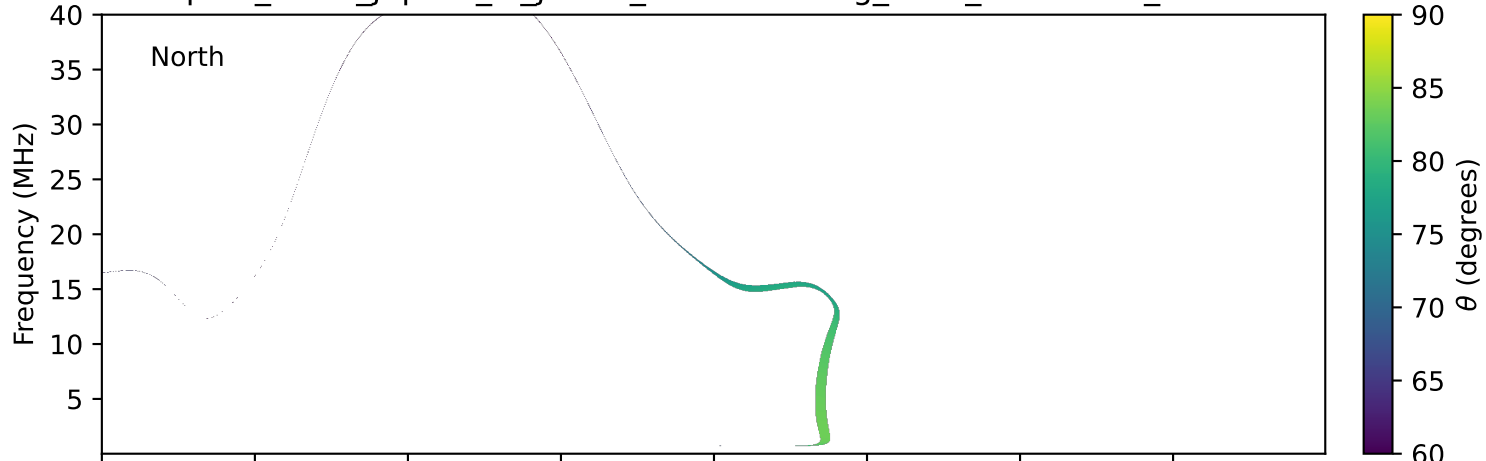
expres_earth_jupiter_io_jrm33_lossc-wid1deg_3kev_20220908_v11.cdf
