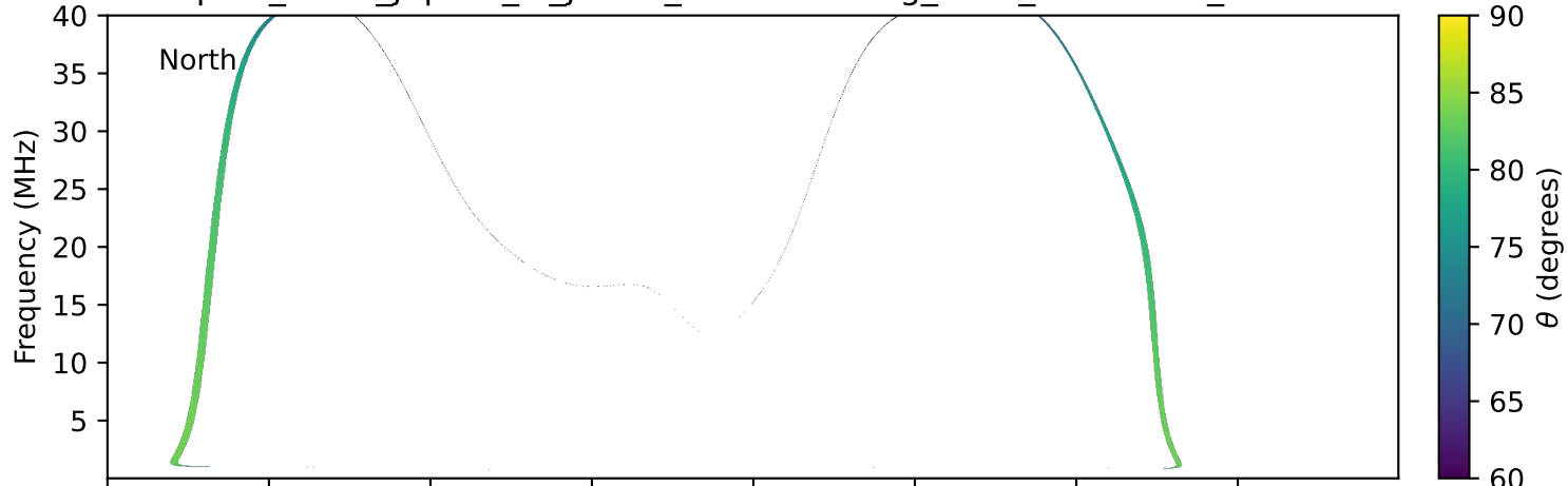
expres_earth_jupiter_io_jrm33_lossc-wid1deg_3kev_20220906_v11.cdf
