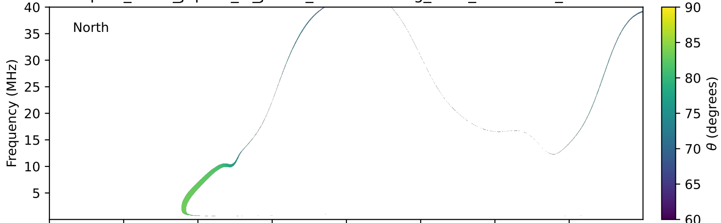
expres_earth_jupiter_io_jrm33_lossc-wid1deg_3kev_20220904_v11.cdf
