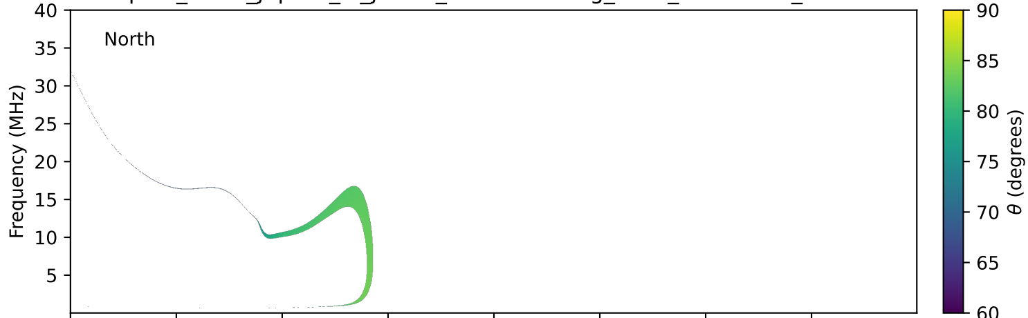
expres_earth_jupiter_io_jrm33_lossc-wid1deg_3kev_20220903_v11.cdf
