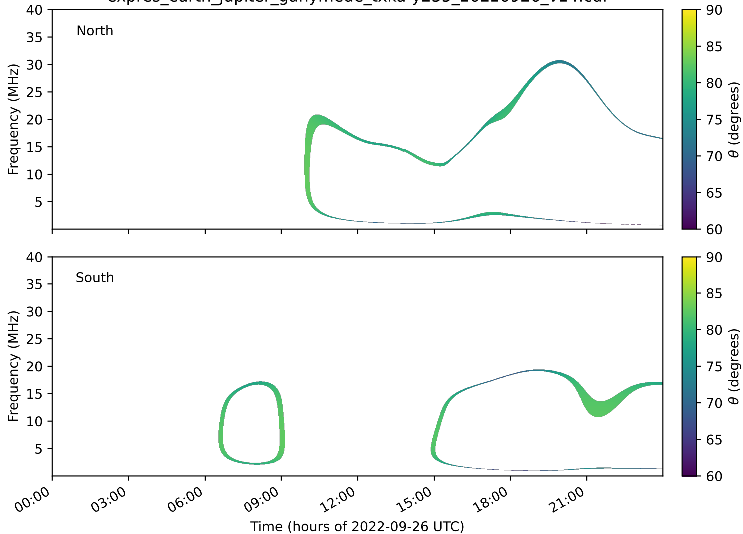
expres_earth_jupiter_ganymede_txka-y235_20220926_v14.cdf
