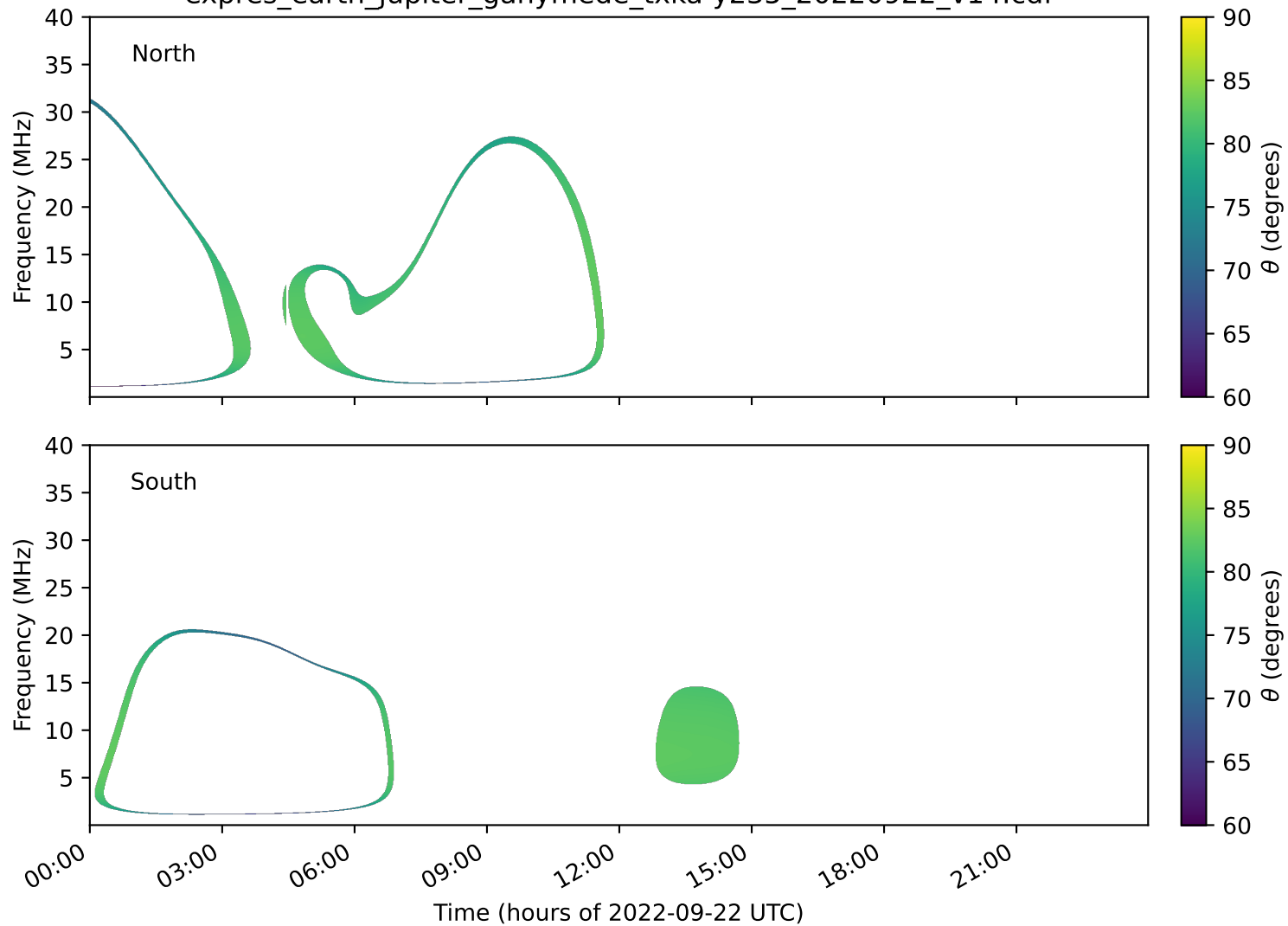
expres_earth_jupiter_ganymede_txka-y235_20220922_v14.cdf
