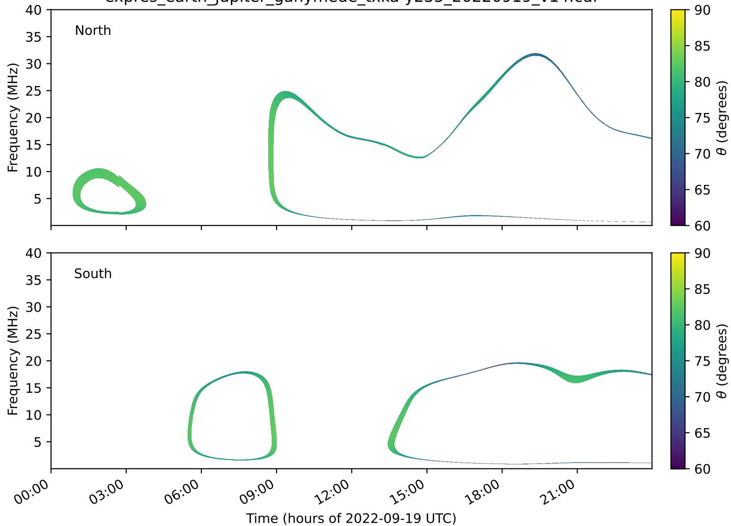
expres_earth_jupiter_ganymede_txka-y235_20220919_v14.cdf
