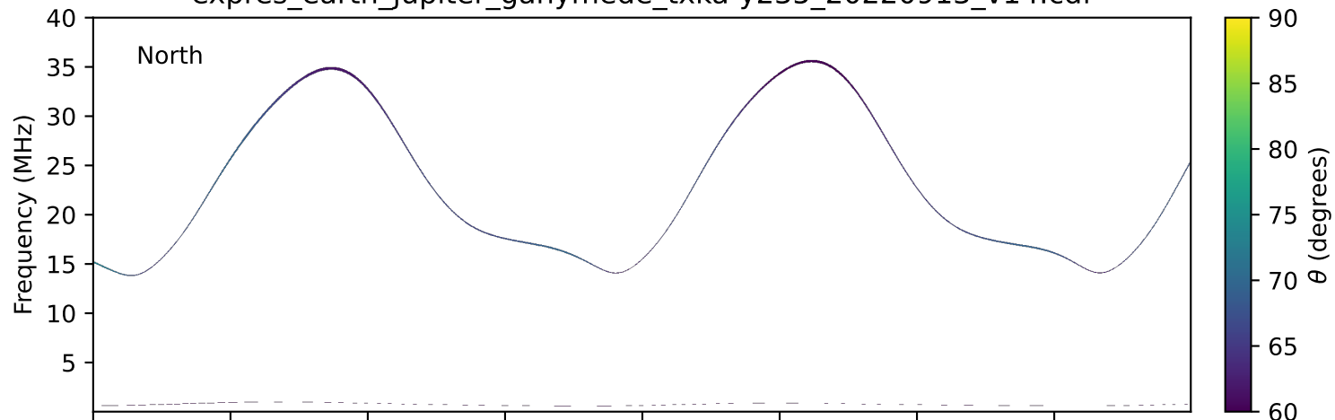
expres_earth_jupiter_ganymede_txka-y235_20220913_v14.cdf
