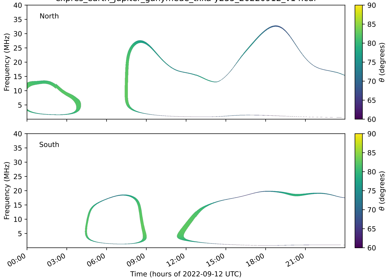
expres_earth_jupiter_ganymede_txka-y235_20220912_v14.cdf
