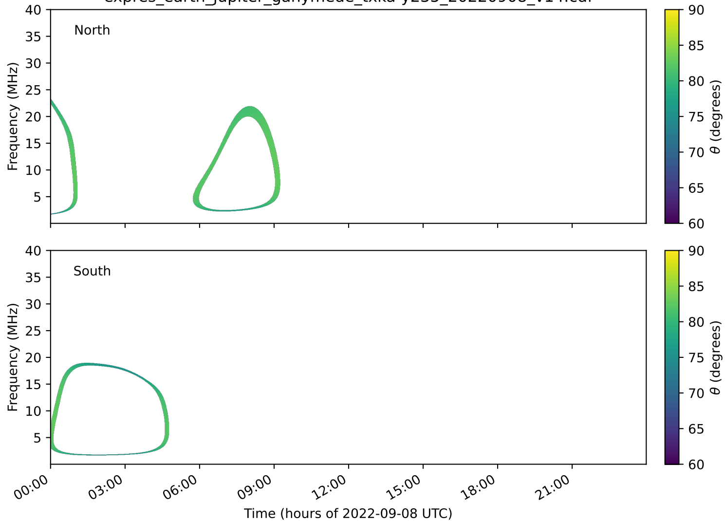
expres_earth_jupiter_ganymede_txka-y235_20220908_v14.cdf
