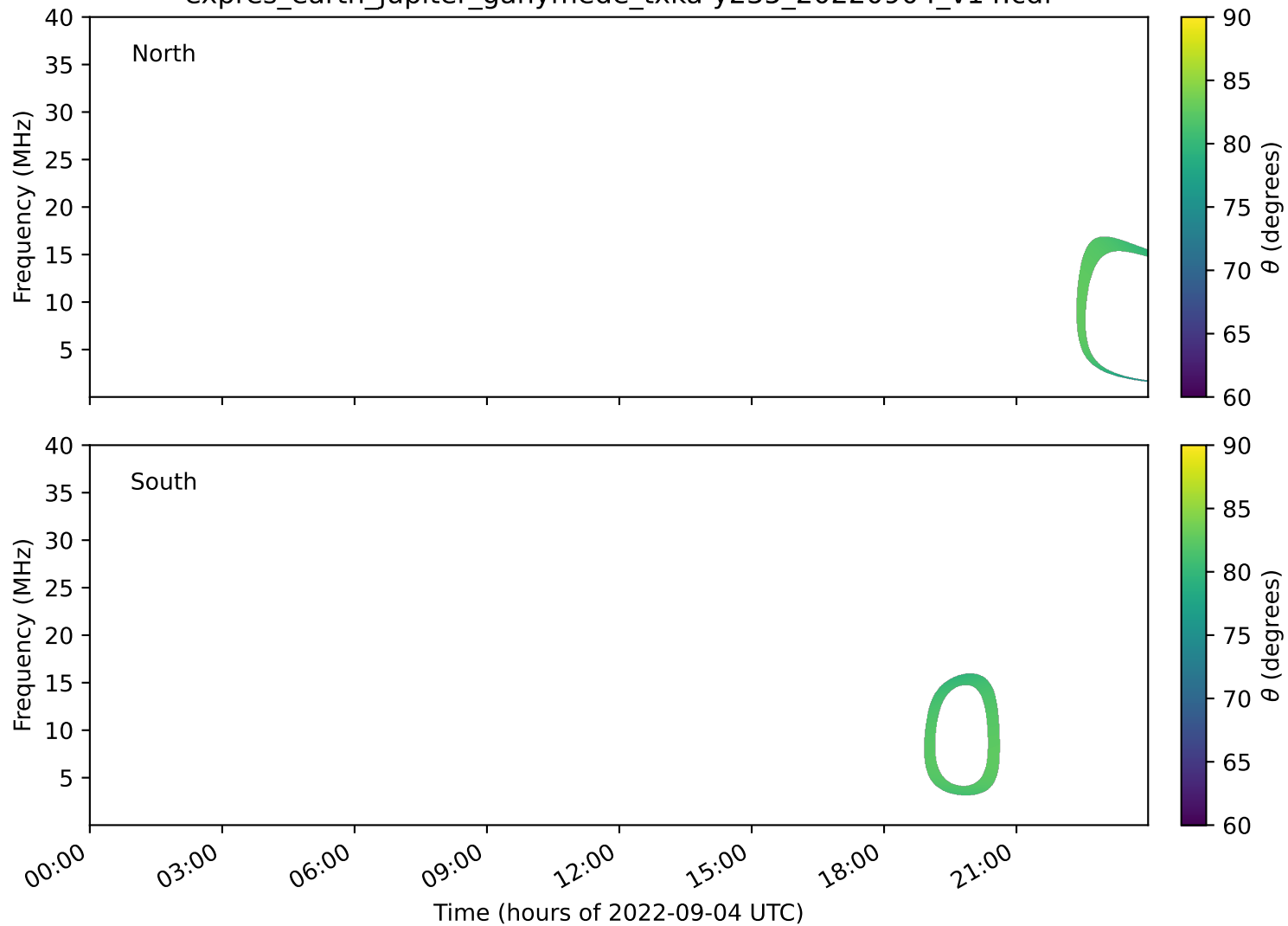
expres_earth_jupiter_ganymede_txka-y235_20220904_v14.cdf
