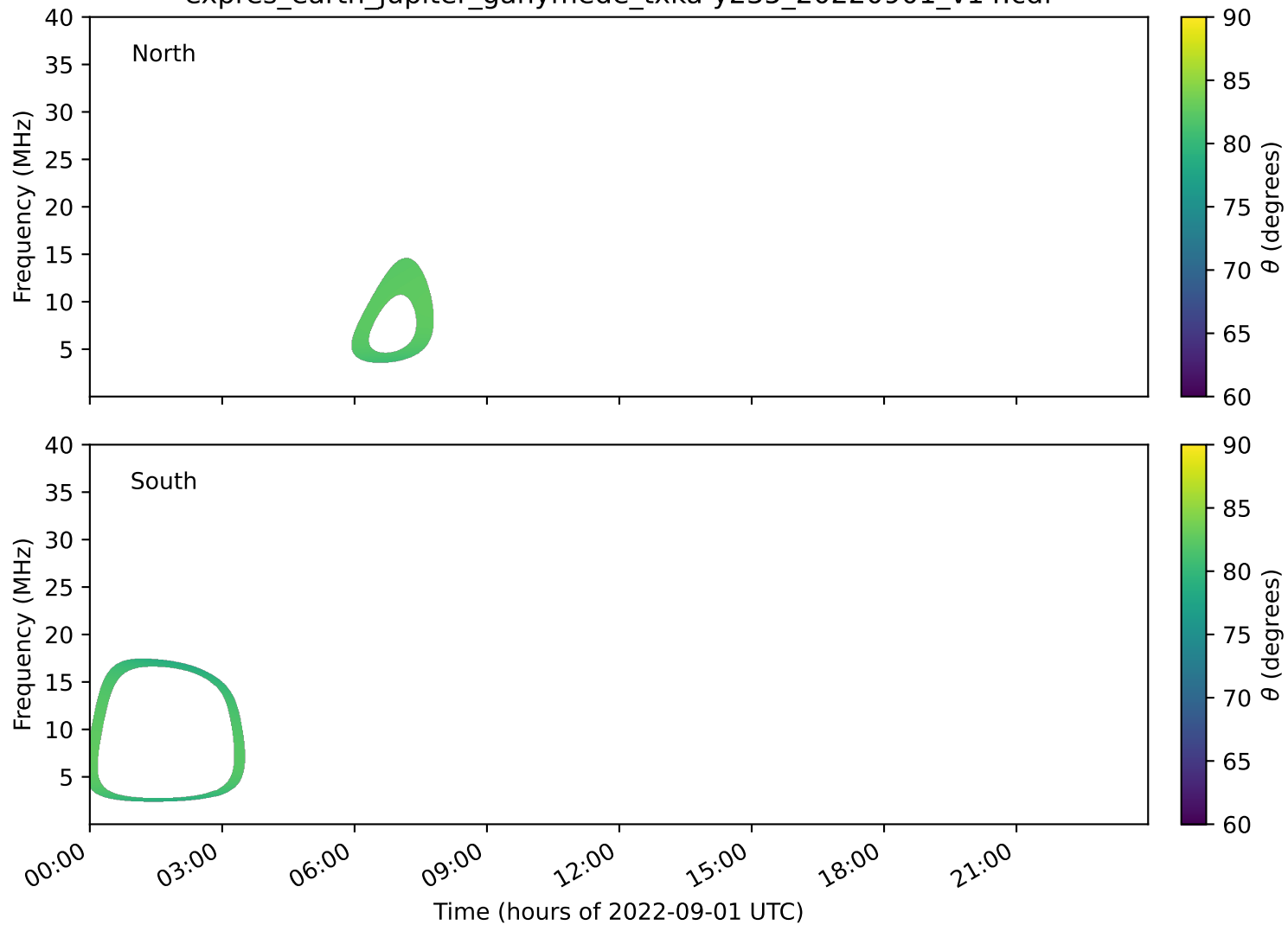
expres_earth_jupiter_ganymede_txka-y235_20220901_v14.cdf
