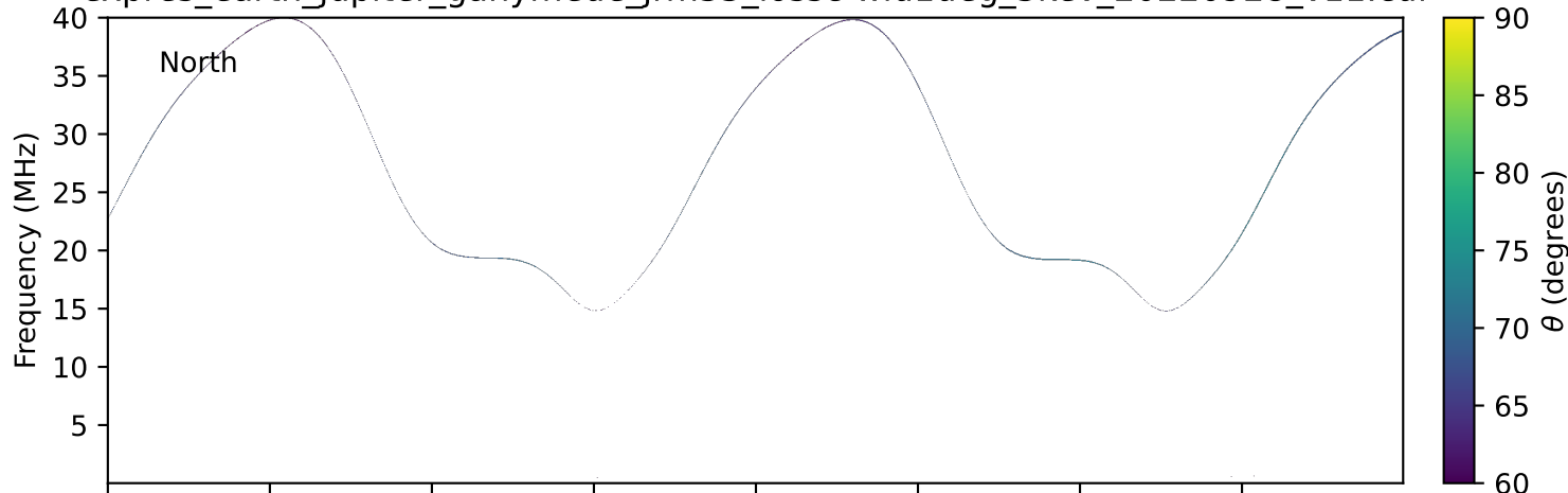
expres_earth_jupiter_ganymede_jrm33_lossc-wid1deg_3kev_20220928_v11.cdf
