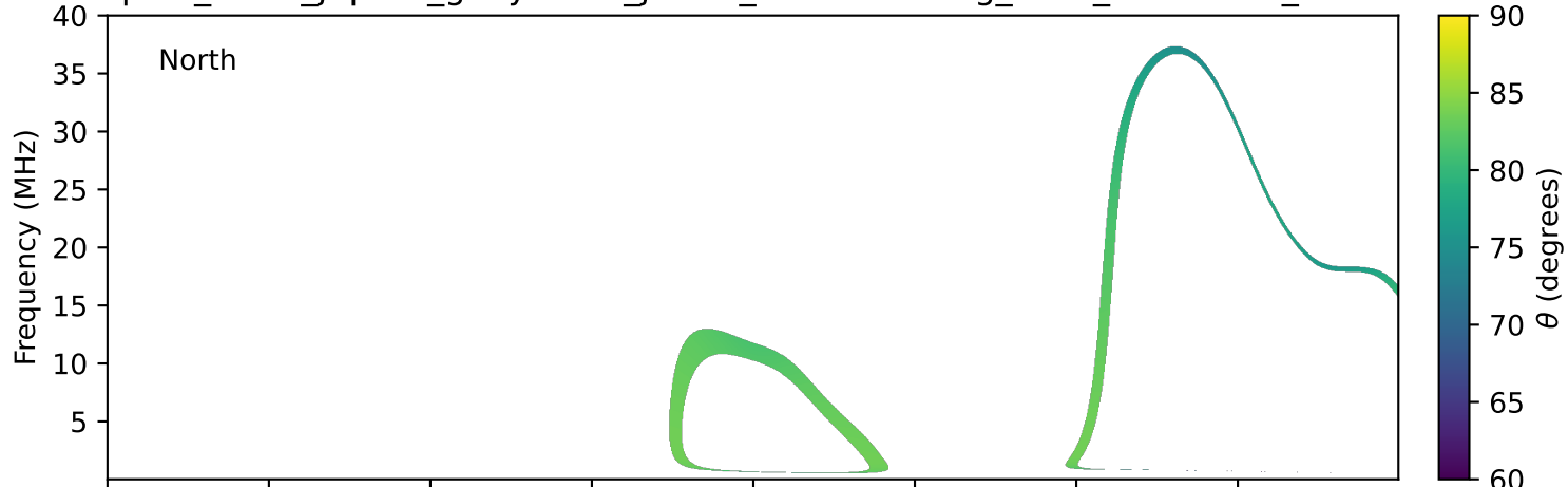
expres_earth_jupiter_ganymede_jrm33_lossc-wid1deg_3kev_20220926_v11.cdf
