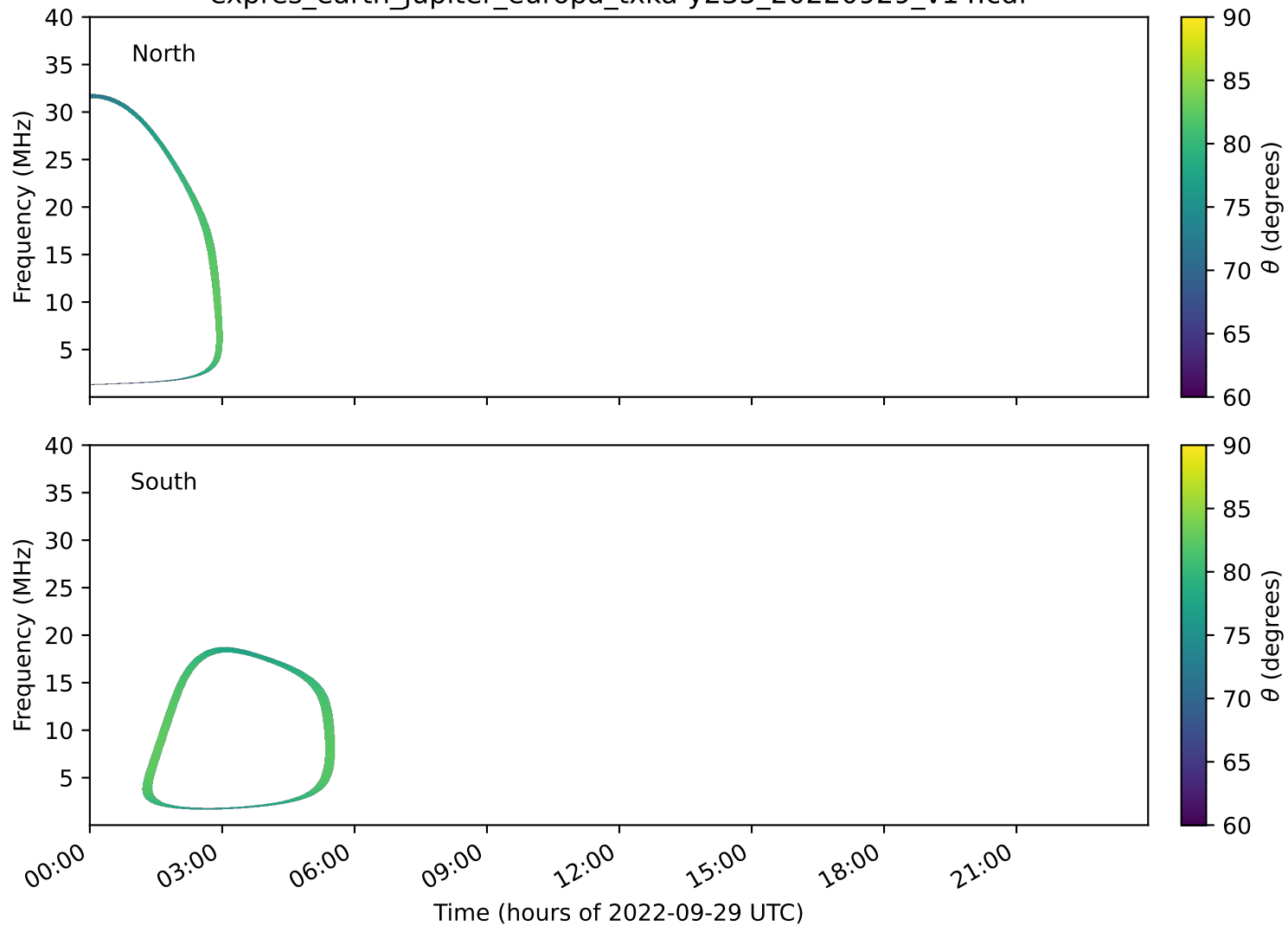
expres_earth_jupiter_europa_txka-y235_20220929_v14.cdf
