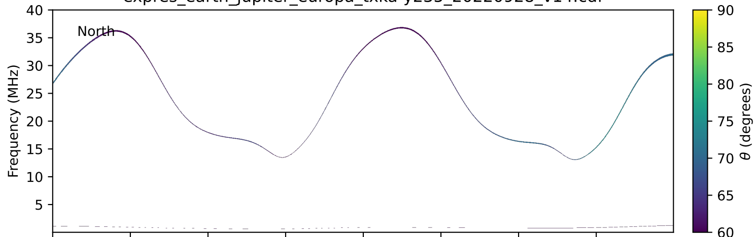
expres_earth_jupiter_europa_txka-y235_20220928_v14.cdf
