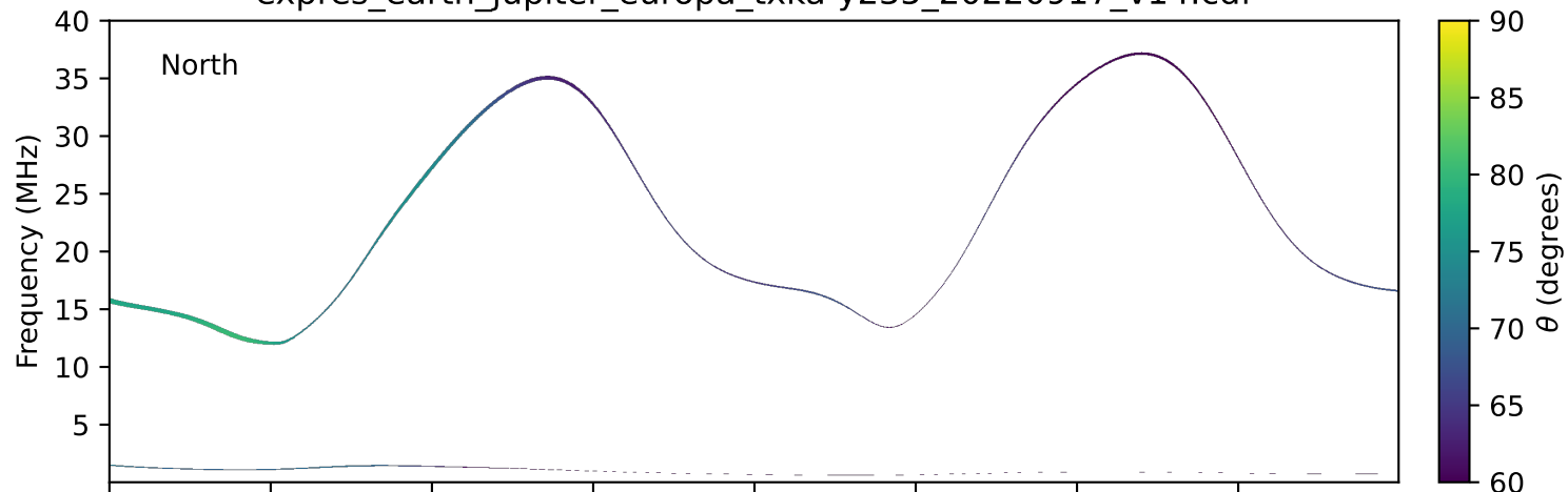
expres_earth_jupiter_europa_txka-y235_20220917_v14.cdf
