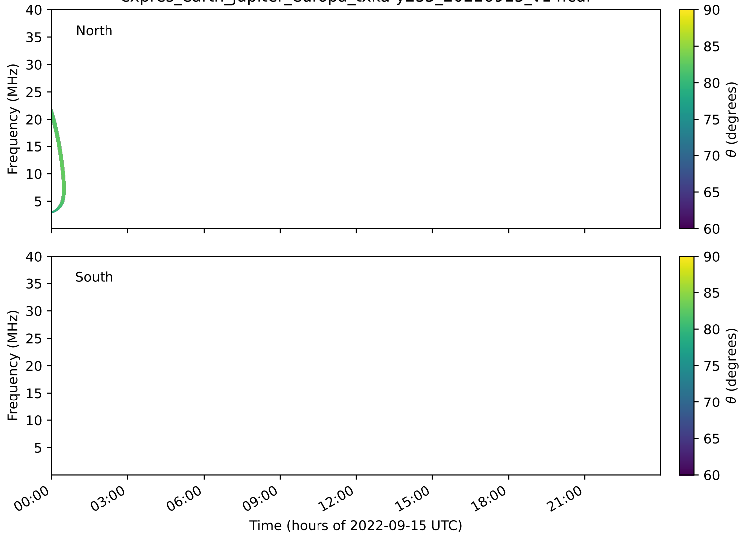
expres_earth_jupiter_europa_txka-y235_20220915_v14.cdf
