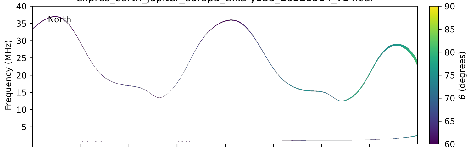
expres_earth_jupiter_europa_txka-y235_20220914_v14.cdf
