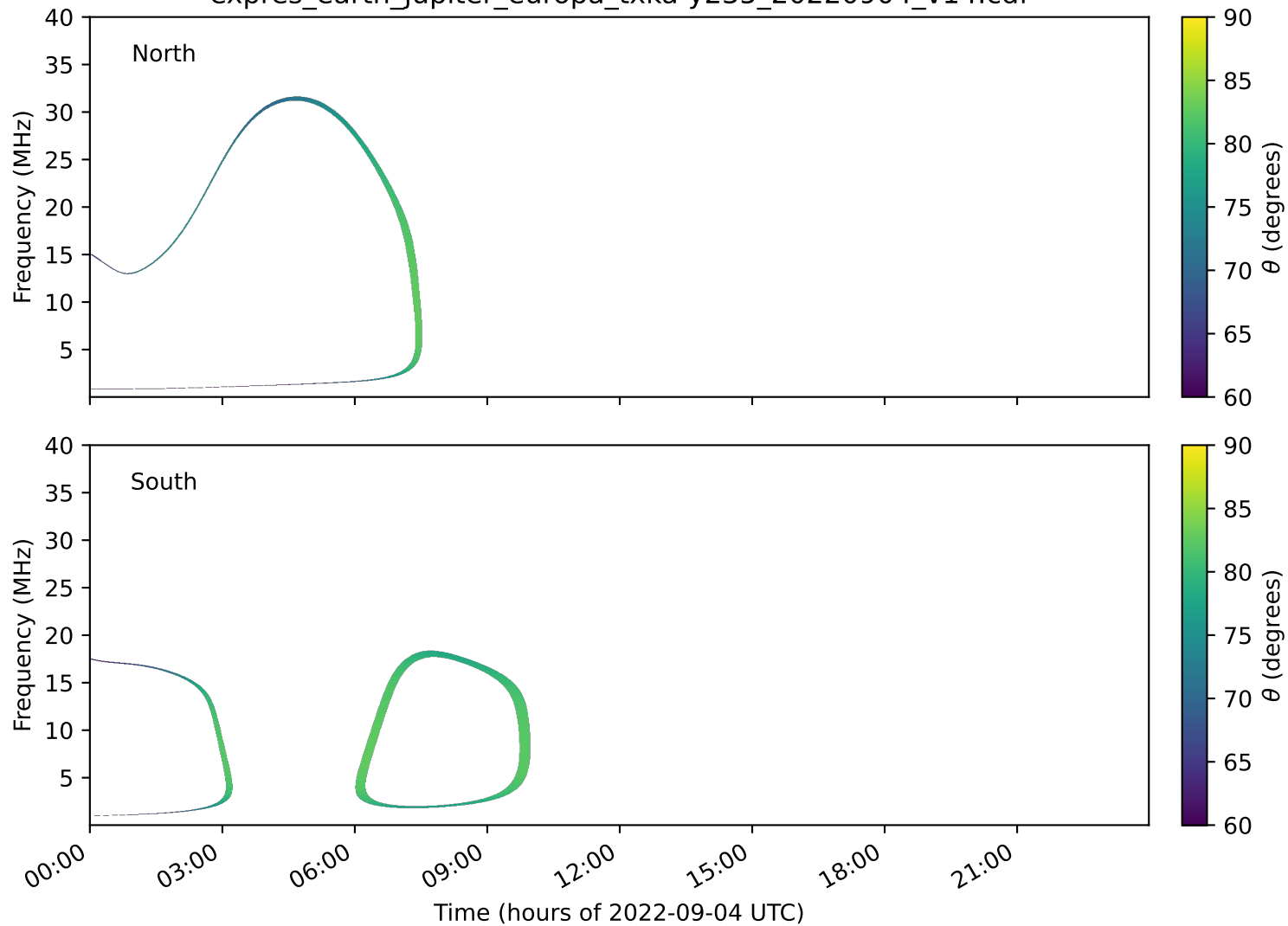
expres_earth_jupiter_europa_txka-y235_20220904_v14.cdf
