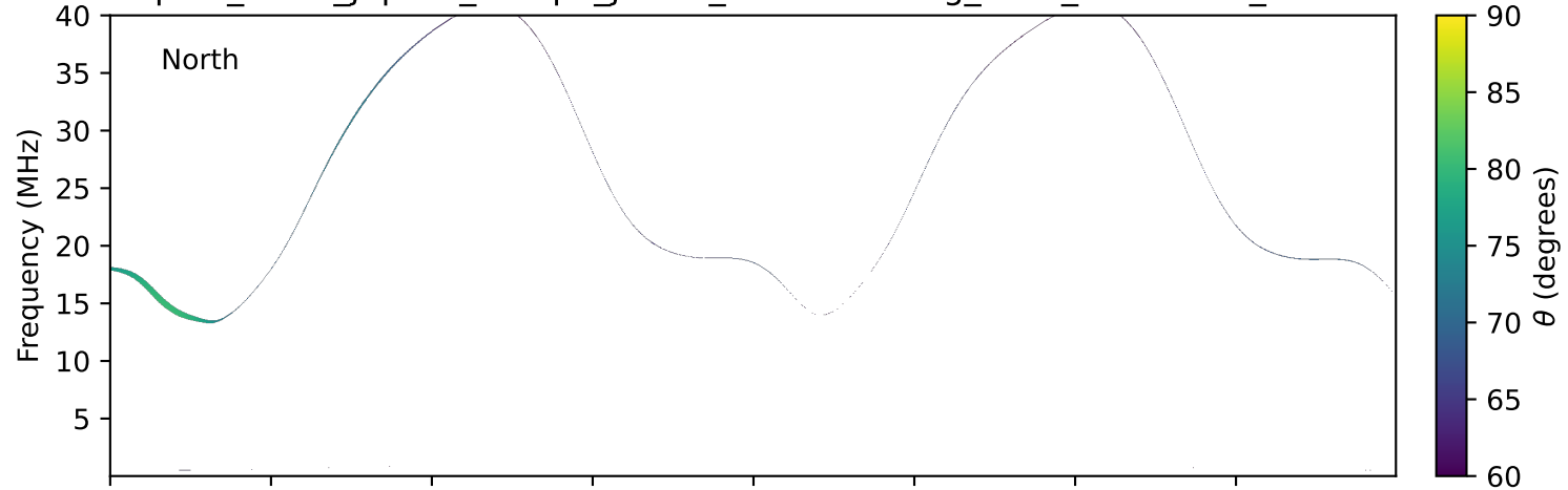
expres_earth_jupiter_europa_jrm33_lossc-wid1deg_3kev_20220903_v11.cdf
