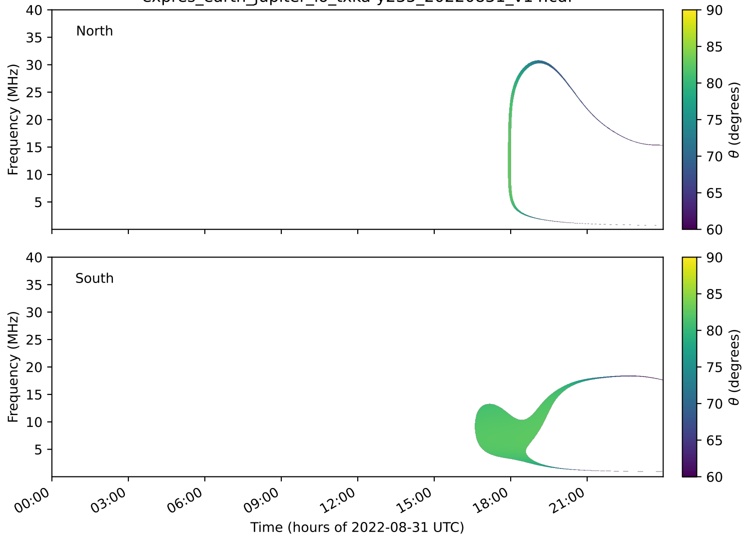
expres_earth_jupiter_io_txka-y235_20220831_v14.cdf
