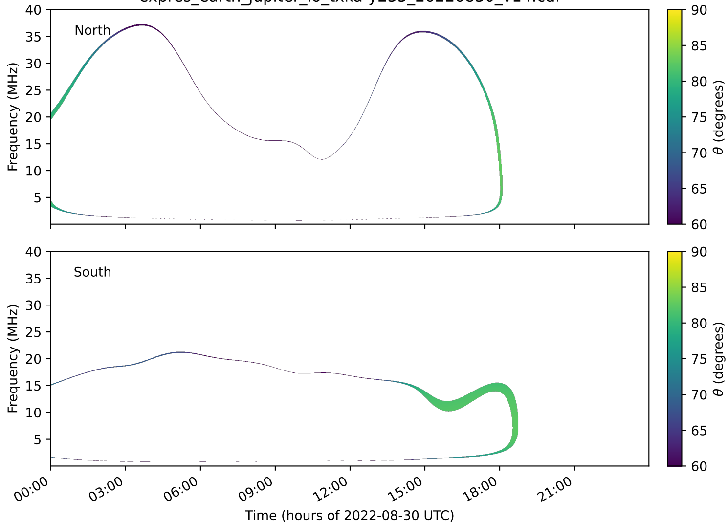
expres_earth_jupiter_io_txka-y235_20220830_v14.cdf
