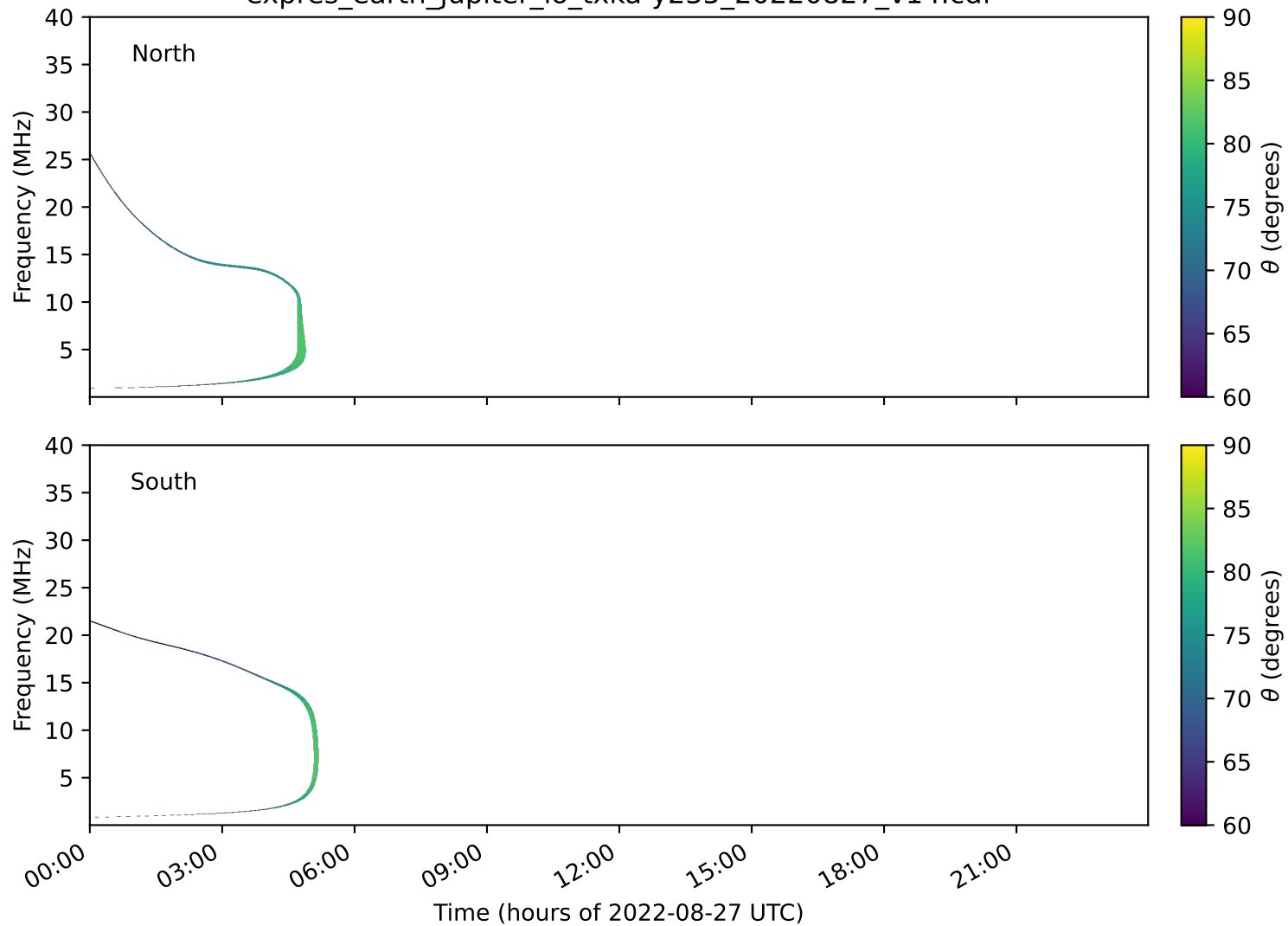
expres_earth_jupiter_io_txka-y235_20220827_v14.cdf
