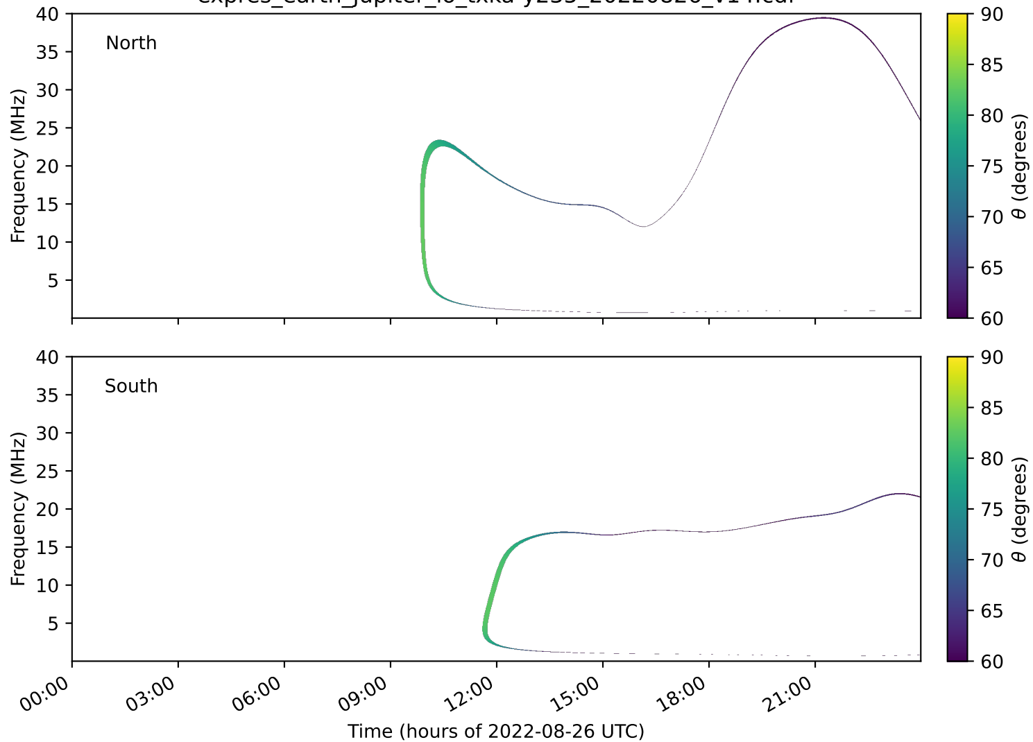
expres_earth_jupiter_io_txka-y235_20220826_v14.cdf
