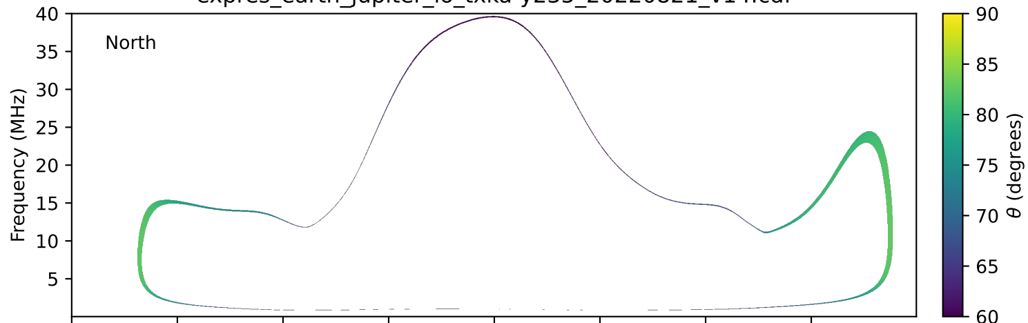
expres_earth_jupiter_io_txka-y235_20220821_v14.cdf
