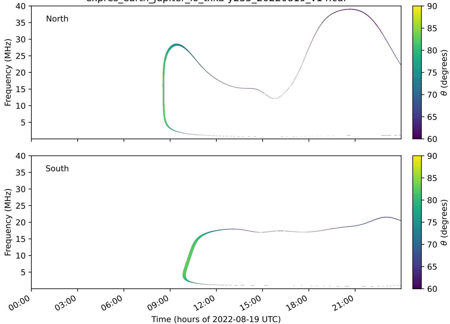
expres_earth_jupiter_io_txka-y235_20220819_v14.cdf
