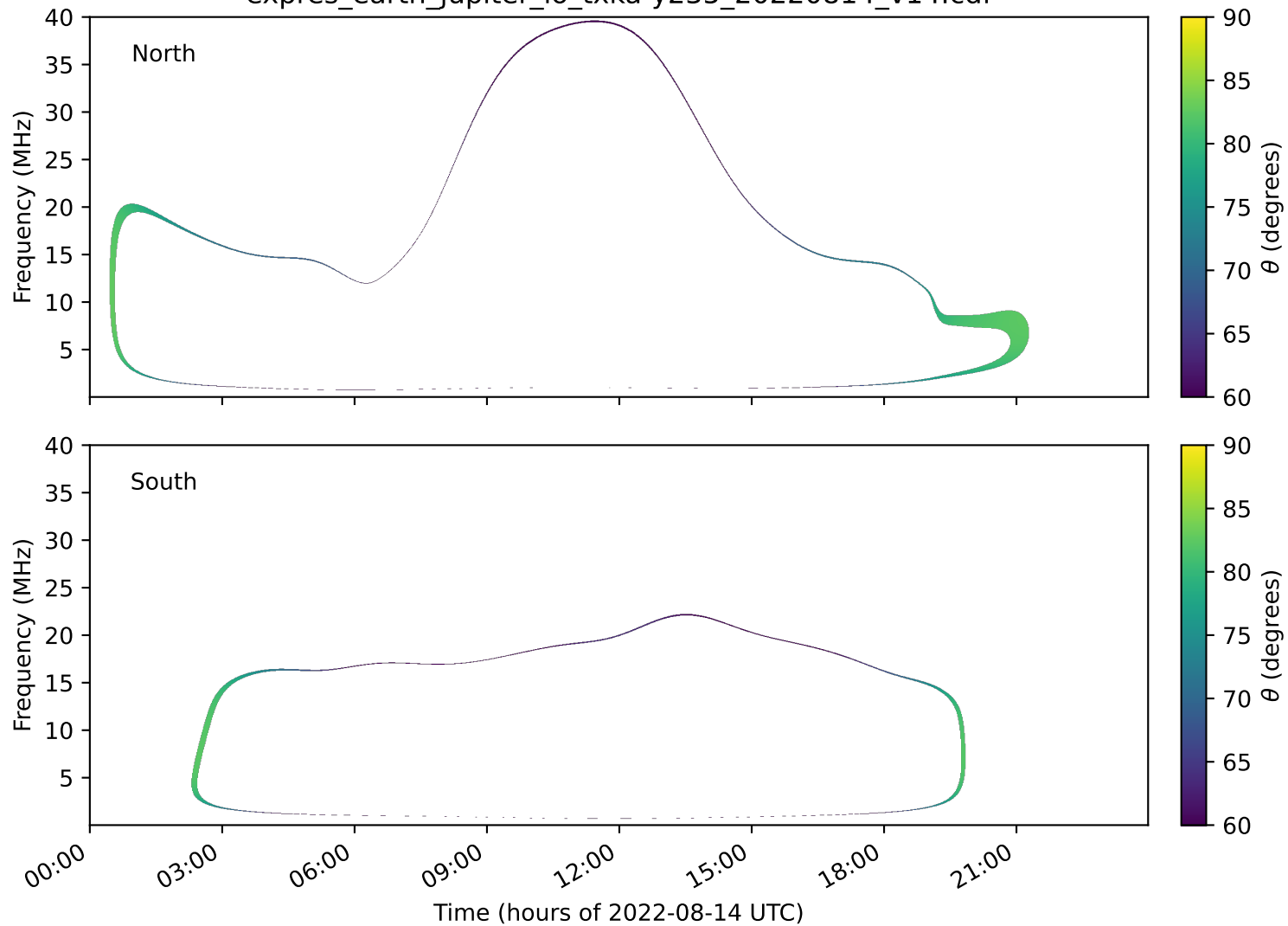
expres_earth_jupiter_io_txka-y235_20220814_v14.cdf
