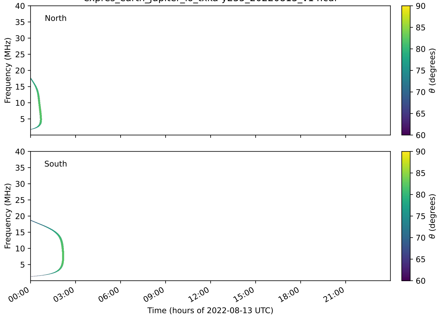
expres_earth_jupiter_io_txka-y235_20220813_v14.cdf
