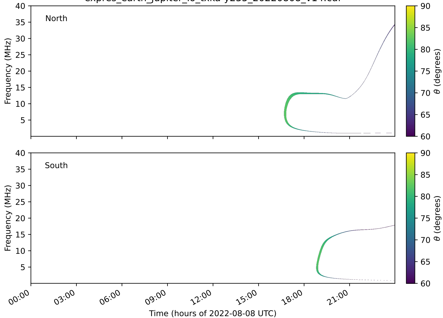
expres_earth_jupiter_io_txka-y235_20220808_v14.cdf
