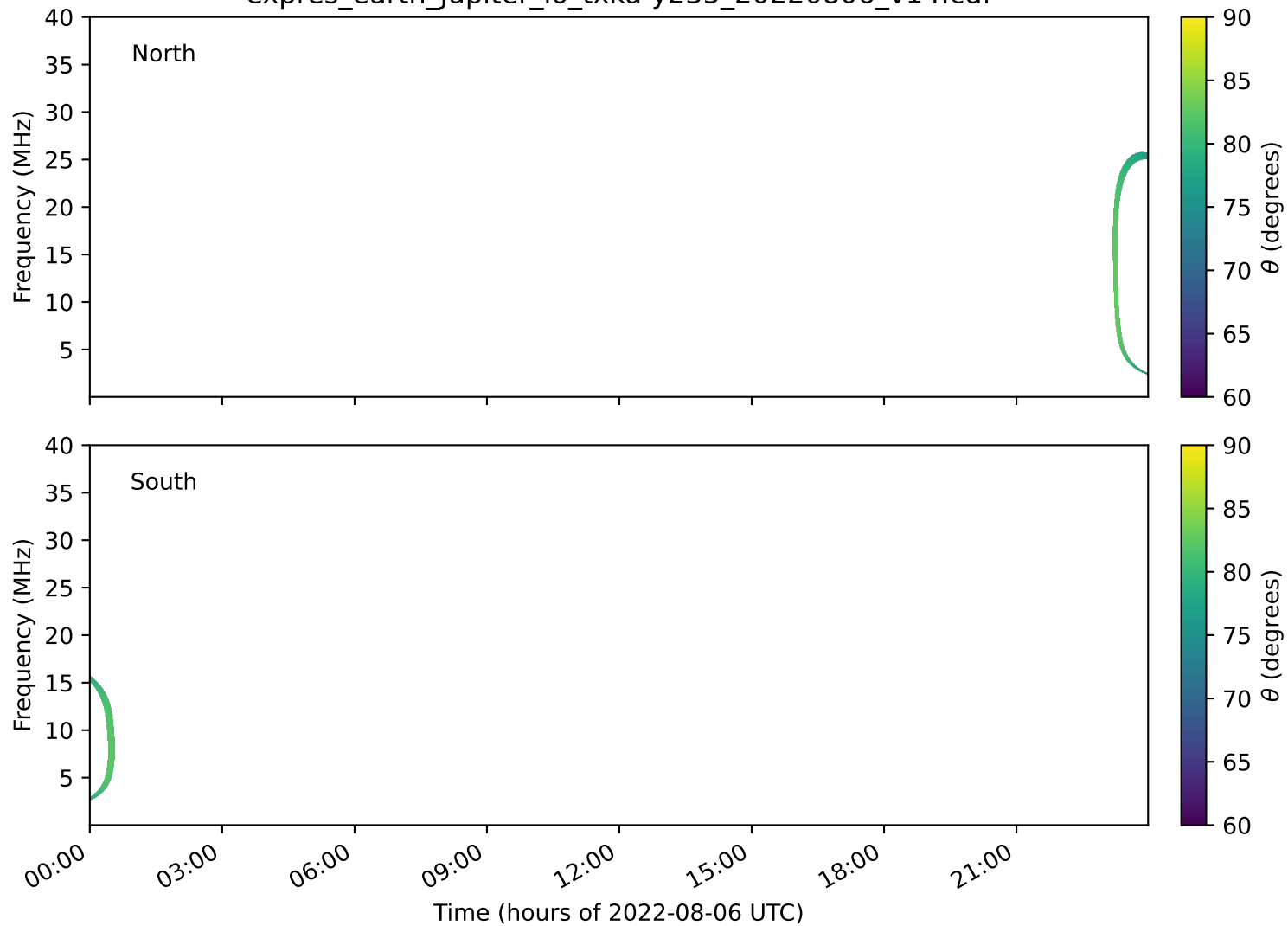
expres_earth_jupiter_io_txka-y235_20220806_v14.cdf
